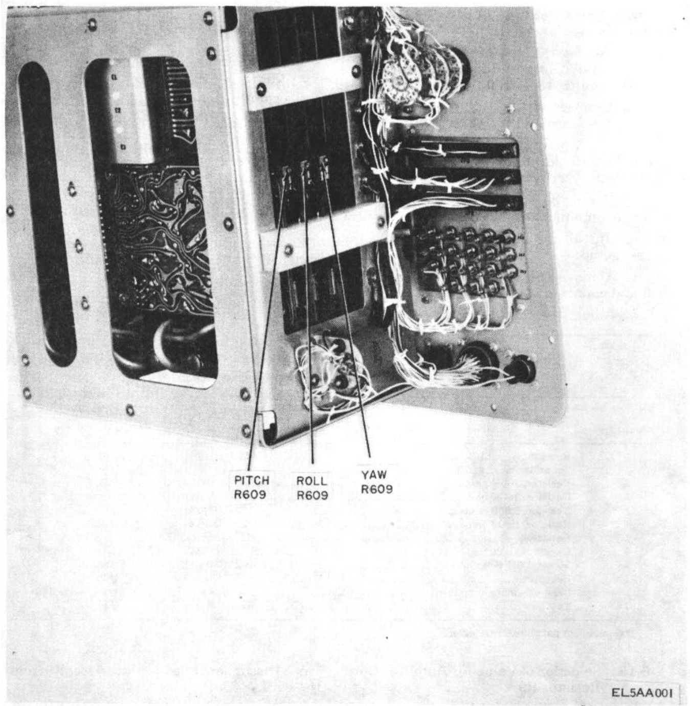
Figure 6-7. Balance resistors location.
