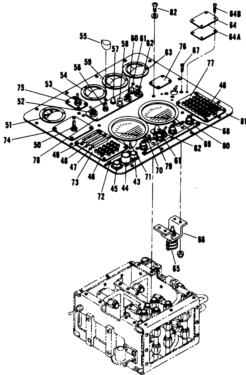
FIGURE 9-1. SAS BENCH TEST SET, EXPLODED VIEW (SHEET 2)
