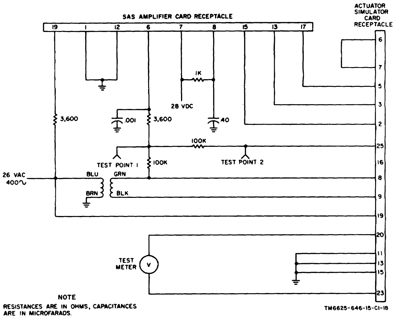
Figure 6-6. Actuator-simulator card, test setup.
