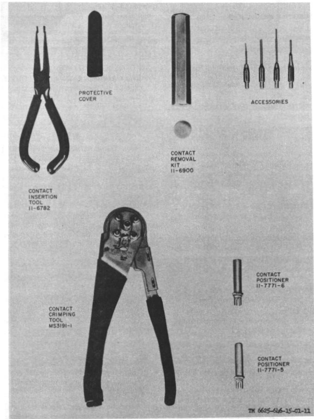
Figure 4-3. Connector contact tools.
