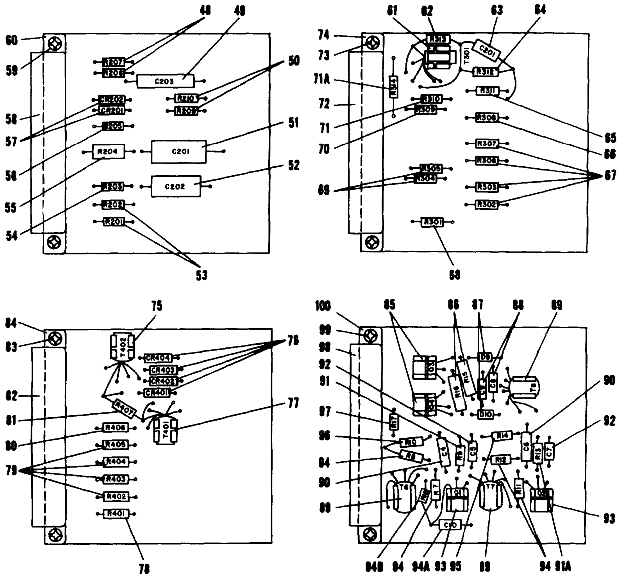
FIGURE 9-2. SAS BENCH TEST SET COMPONENT BOARDS (SHEET 2)
