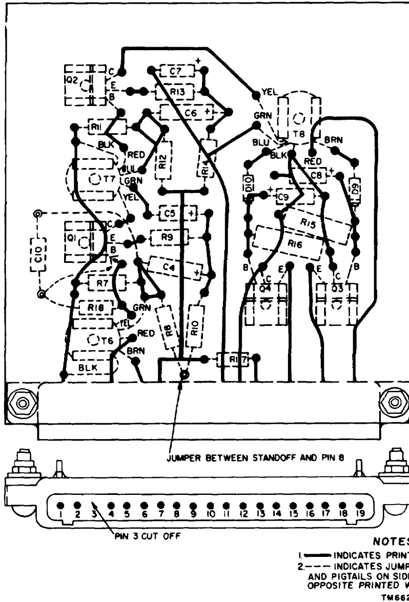
Figure 6-3. Amplifiers card, wiring diagram.
